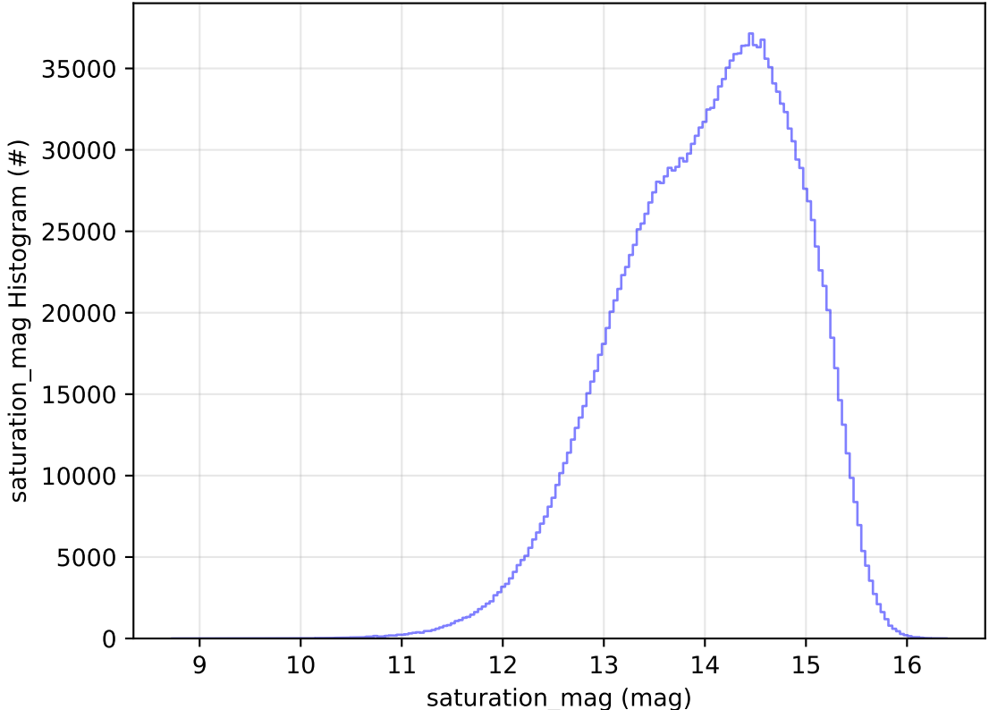
too_elab_r256_d2_ugrizy_v3.4_10yrs WFD all bands: saturation_mag Histogram
