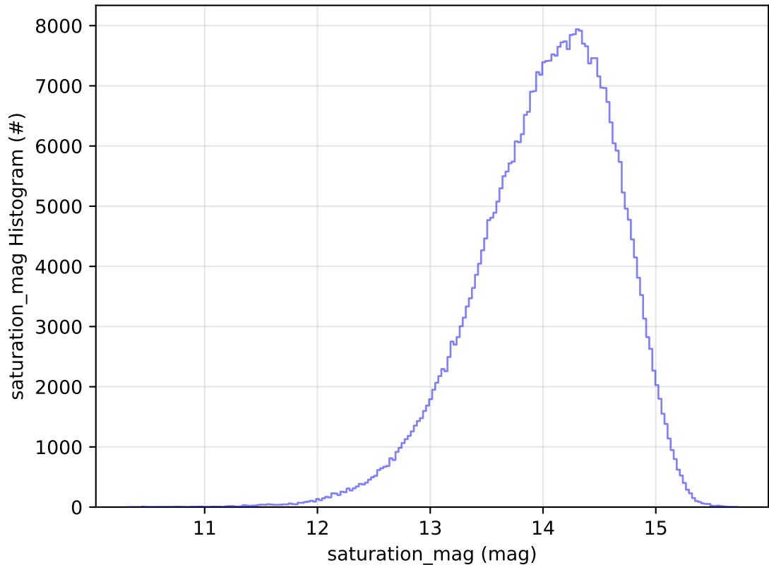
too_elab_r256_d2_ugrizy_v3.4_10yrs All sky z band: saturation_mag Histogram
