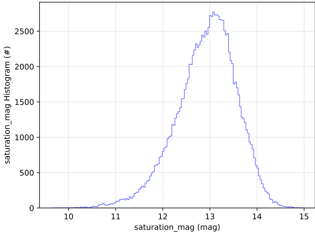
too_elab_r256_d2_ugrizy_v3.4_10yrs All sky u band: saturation_mag Histogram
