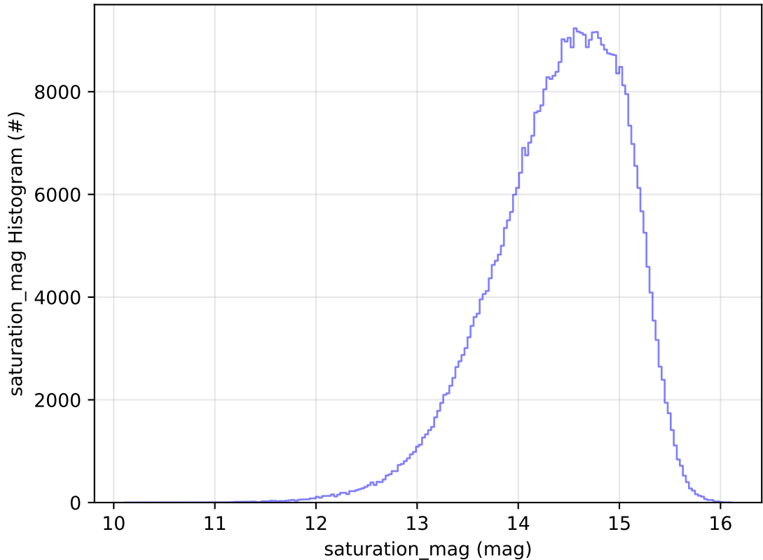
too_elab_r256_d2_ugrizy_v3.4_10yrs All sky i band: saturation_mag Histogram
