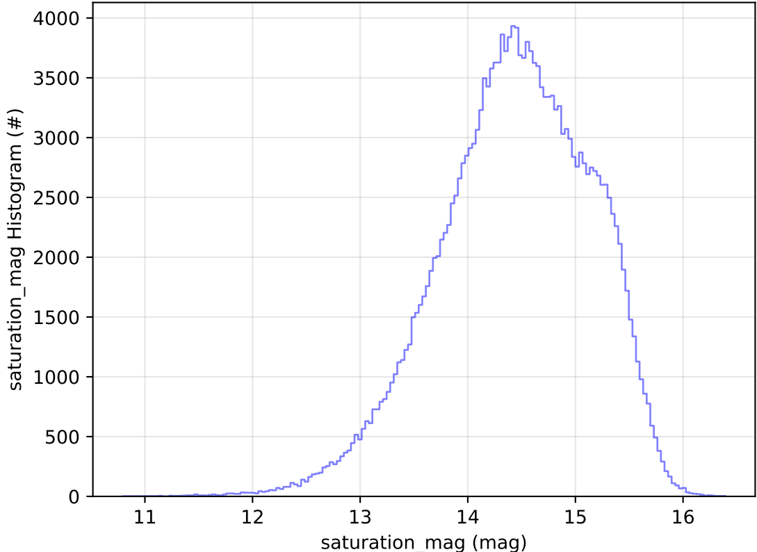
too_elab_r256_d2_ugrizy_v3.4_10yrs All sky g band: saturation_mag Histogram
