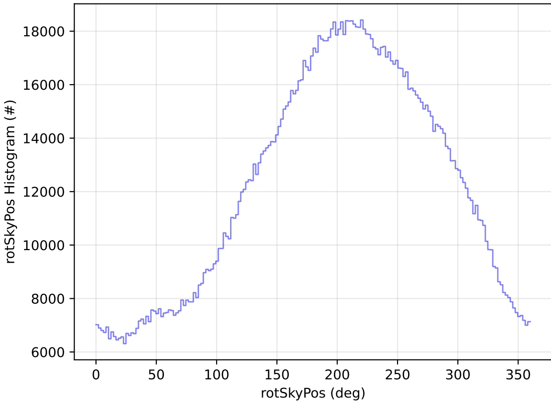
too_elab_r256_d2_ugrizy_v3.4_10yrs WFD all bands: rotSkyPos Histogram
