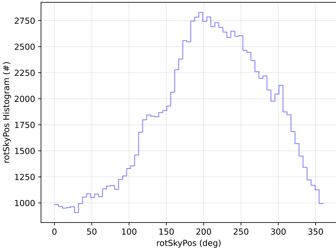
too_elab_r256_d2_ugrizy_v3.4_10yrs All sky u band: rotSkyPos Histogram
