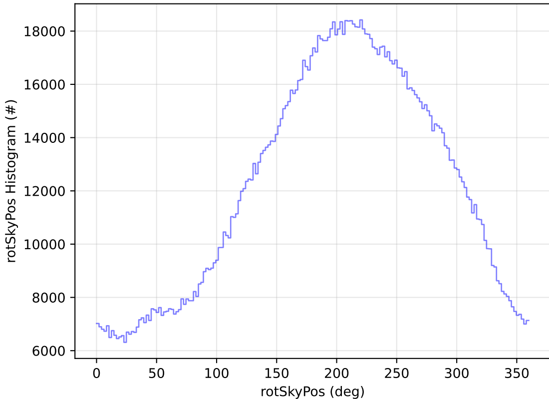
too_elab_r256_d2_ugrizy_v3.4_10yrs All sky all bands: rotSkyPos Histogram
