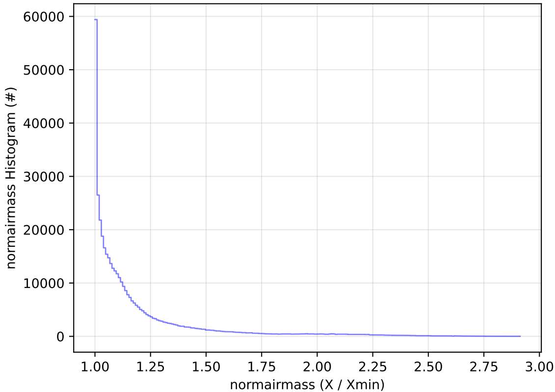
too_elab_r256_d2_ugrizy_v3.4_10yrs WFD z band: normairmass Histogram
