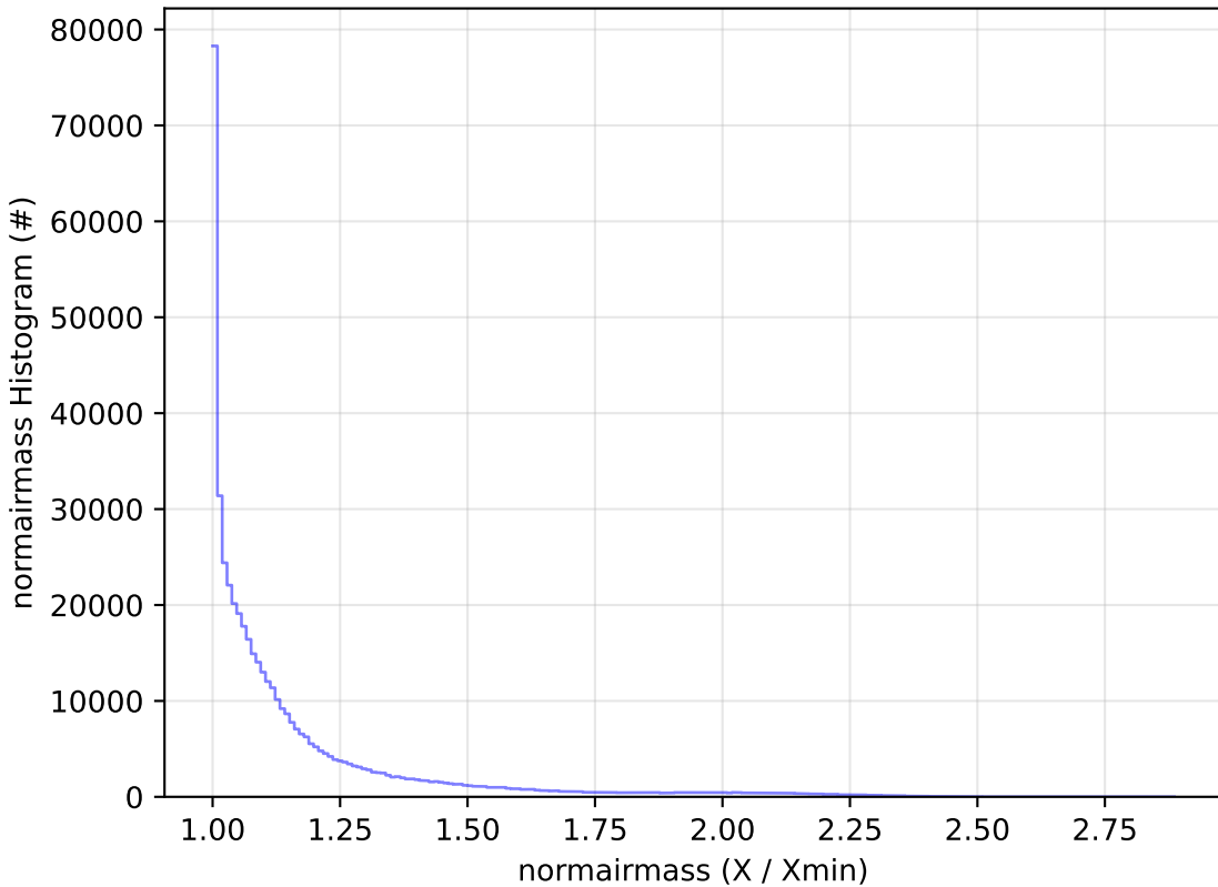
too_elab_r256_d2_ugrizy_v3.4_10yrs WFD r band: normairmass Histogram
