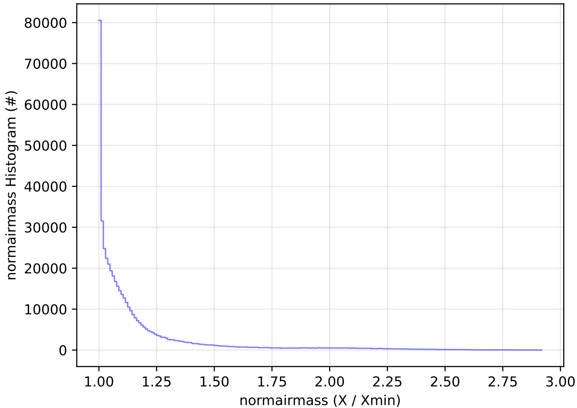
too_elab_r256_d2_ugrizy_v3.4_10yrs WFD i band: normairmass Histogram
