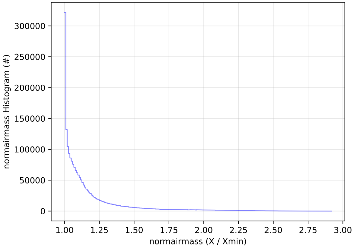
too_elab_r256_d2_ugrizy_v3.4_10yrs WFD all bands: normairmass Histogram
