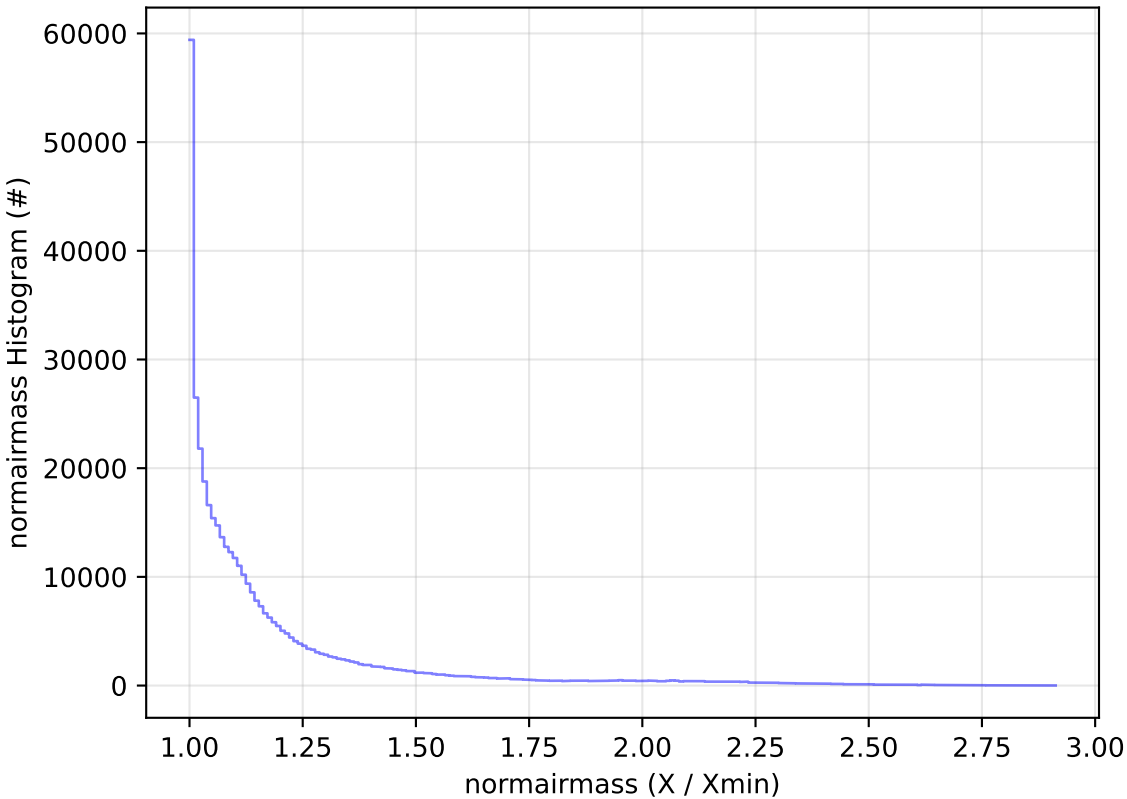
too_elab_r256_d2_ugrizy_v3.4_10yrs All sky z band: normairmass Histogram
