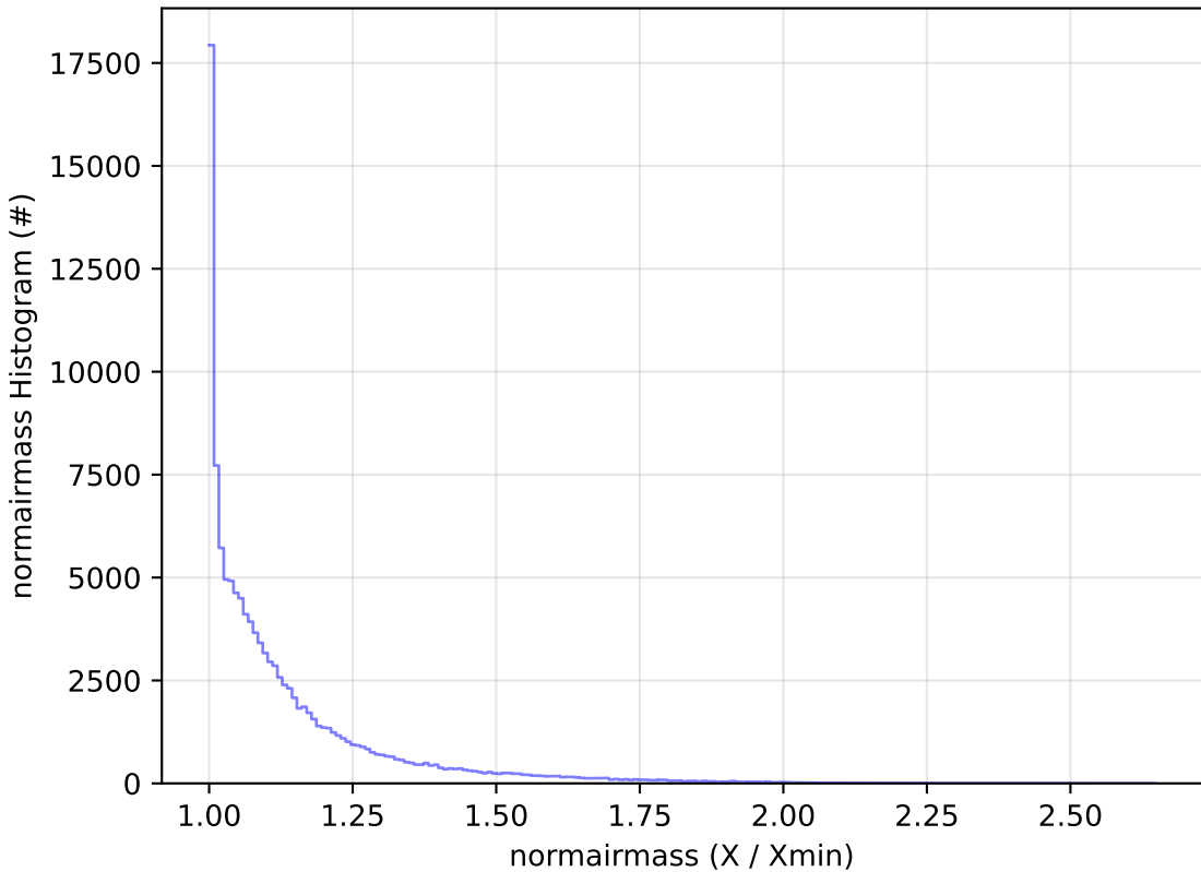
too_elab_r256_d2_ugrizy_v3.4_10yrs All sky u band: normairmass Histogram
