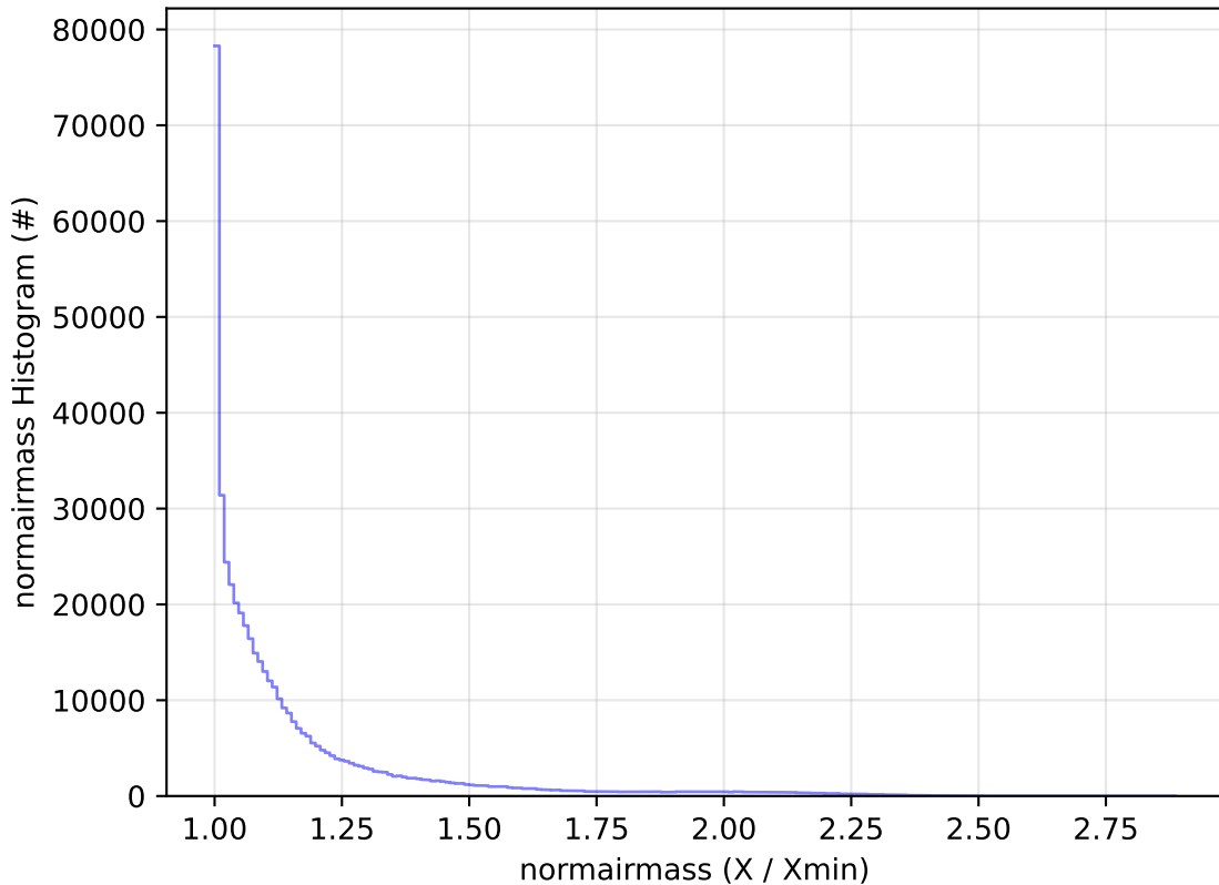
too_elab_r256_d2_ugrizy_v3.4_10yrs All sky r band: normairmass Histogram
