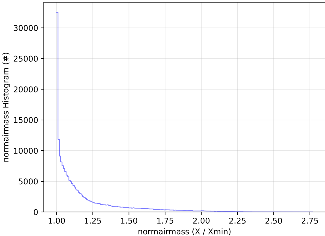
too_elab_r256_d2_ugrizy_v3.4_10yrs All sky g band: normairmass Histogram
