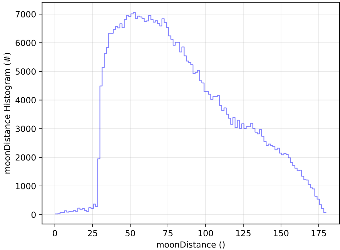
too_elab_r256_d2_ugrizy_v3.4_10yrs WFD z band: moonDistance Histogram
