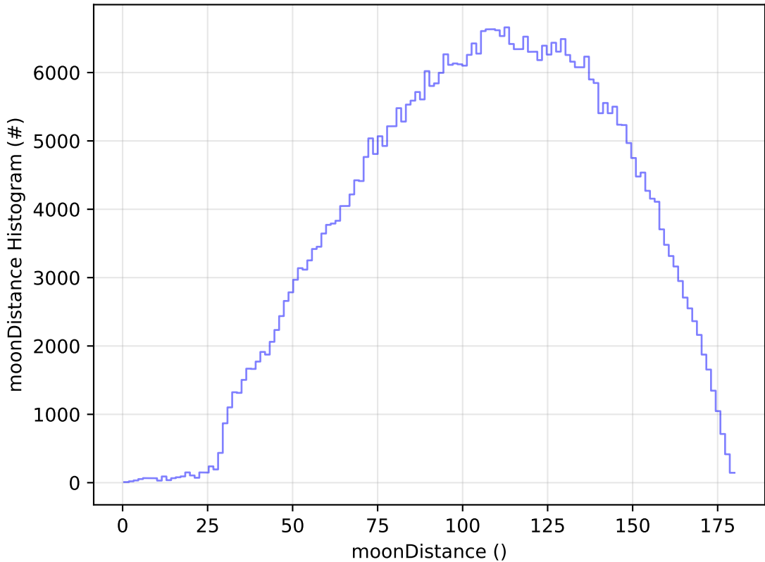
too_elab_r256_d2_ugrizy_v3.4_10yrs WFD r band: moonDistance Histogram
