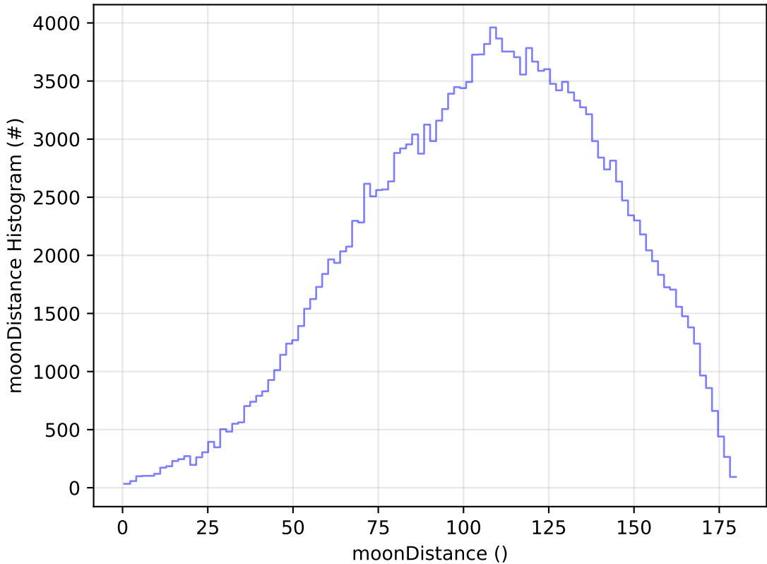
too_elab_r256_d2_ugrizy_v3.4_10yrs WFD g band: moonDistance Histogram
