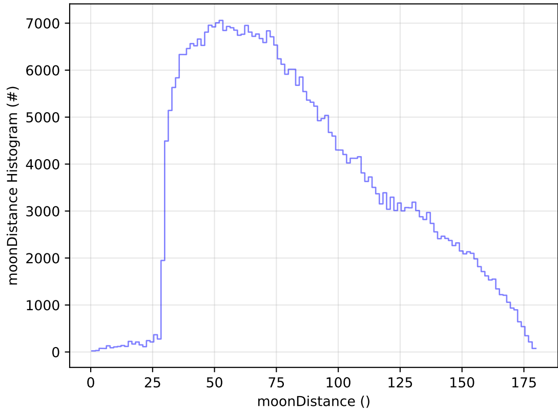
too_elab_r256_d2_ugrizy_v3.4_10yrs All sky z band: moonDistance Histogram
