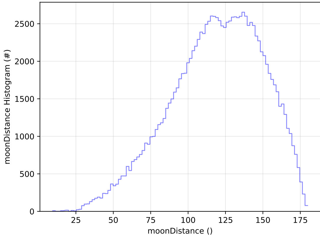
too_elab_r256_d2_ugrizy_v3.4_10yrs All sky u band: moonDistance Histogram
