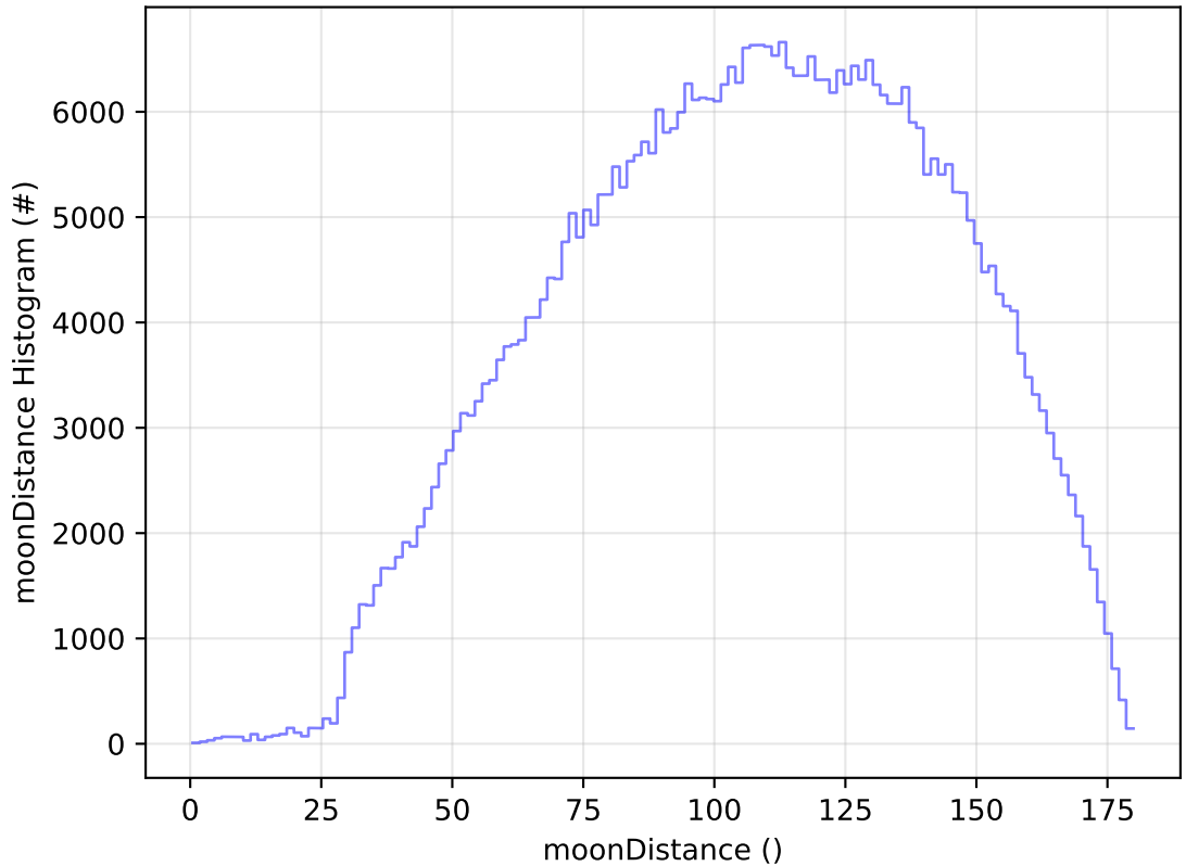
too_elab_r256_d2_ugrizy_v3.4_10yrs All sky r band: moonDistance Histogram
