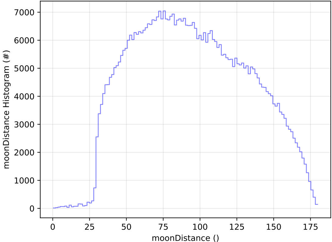
too_elab_r256_d2_ugrizy_v3.4_10yrs All sky i band: moonDistance Histogram
