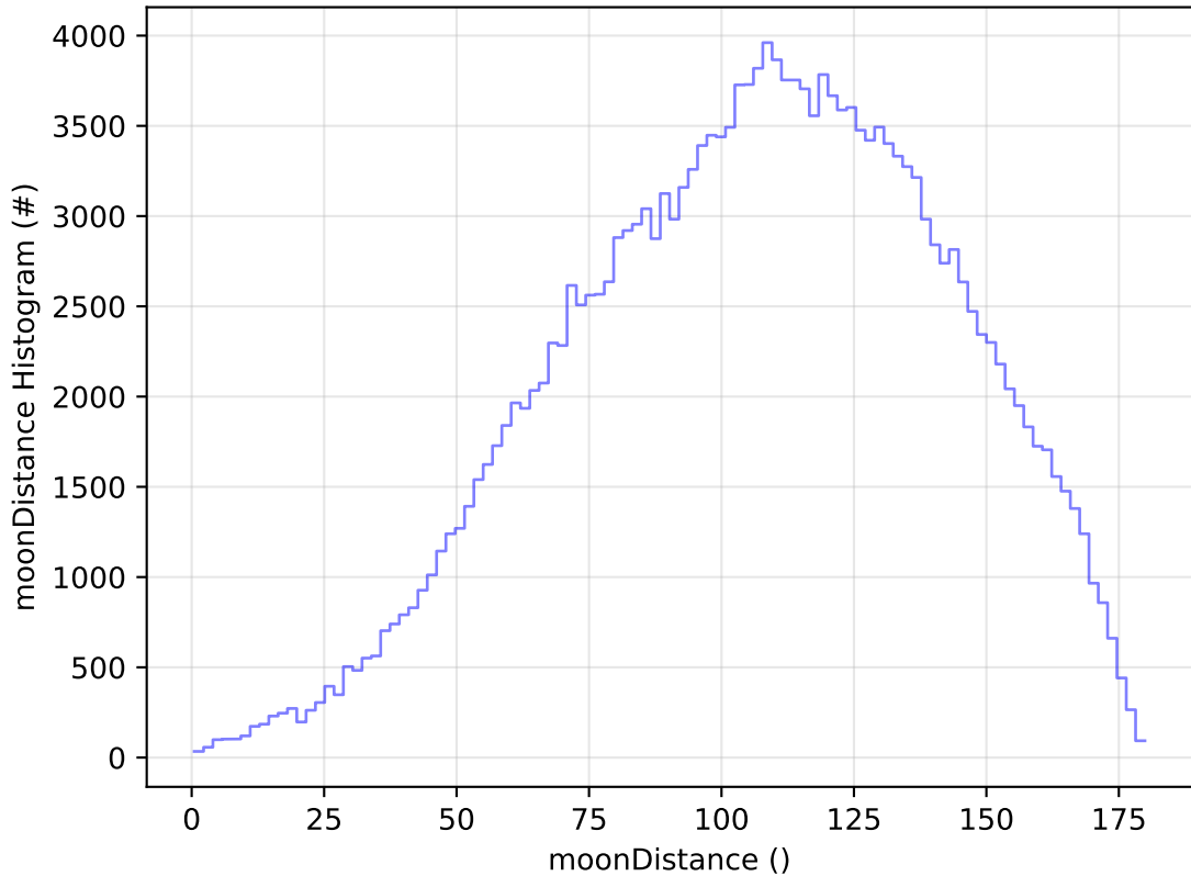
too_elab_r256_d2_ugrizy_v3.4_10yrs All sky g band: moonDistance Histogram
