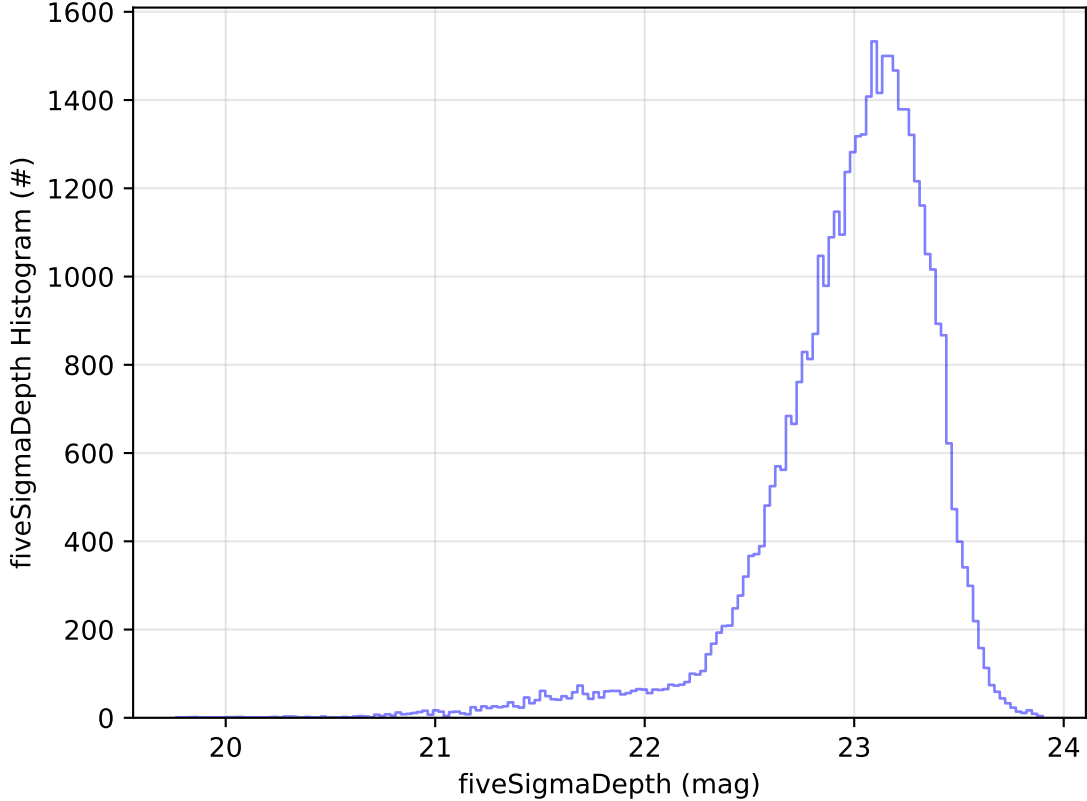
too_elab_r256_d2_ugrizy_v3.4_10yrs Yr 1 z band: fiveSigmaDepth Histogram
