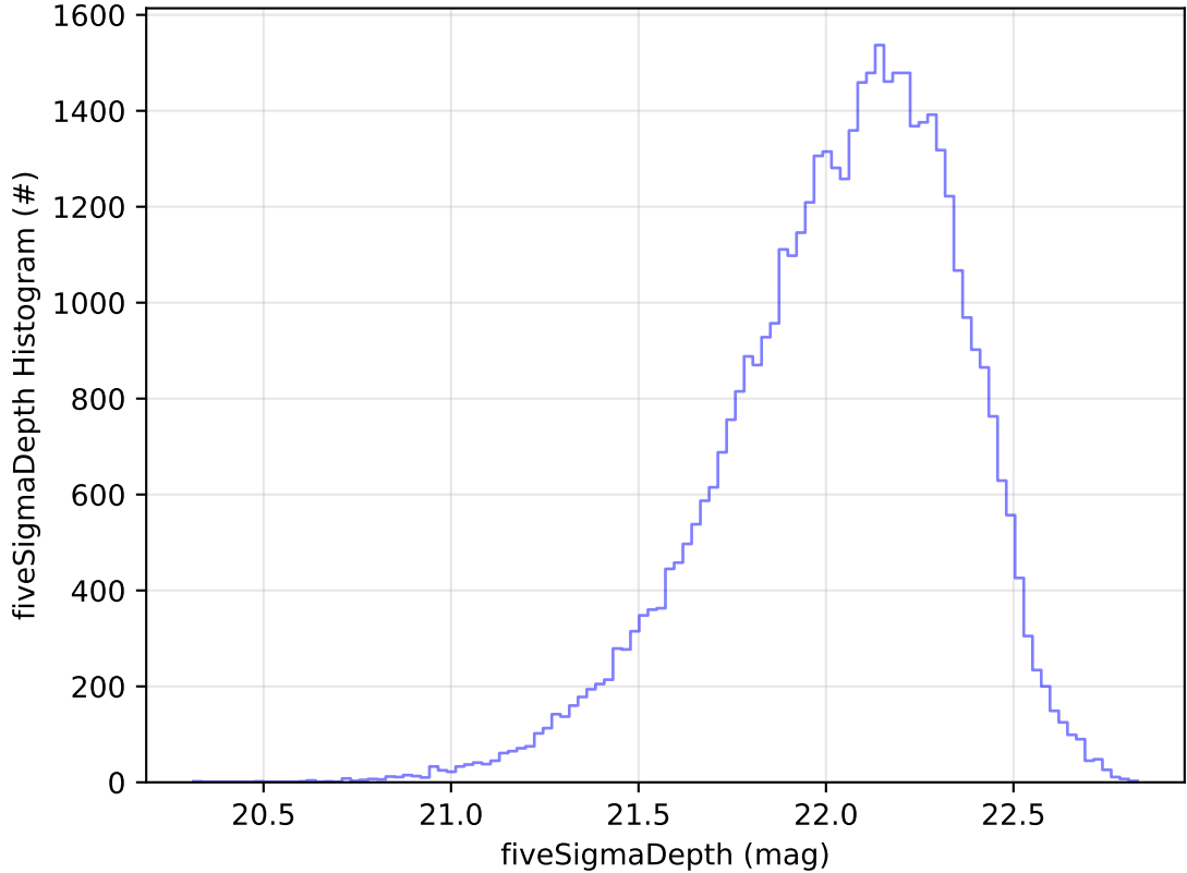
too_elab_r256_d2_ugrizy_v3.4_10yrs Yr 1 y band: fiveSigmaDepth Histogram
