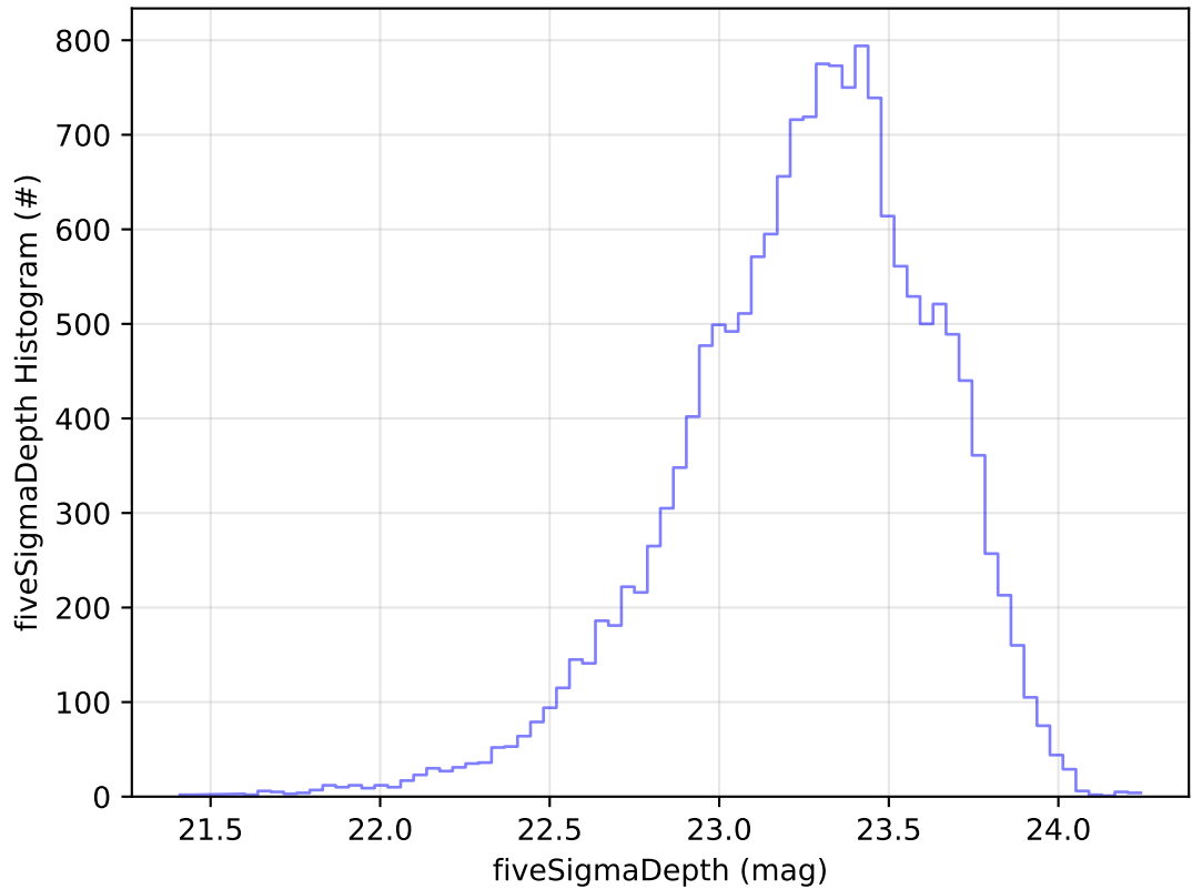
too_elab_r256_d2_ugrizy_v3.4_10yrs Yr 1 u band: fiveSigmaDepth Histogram
