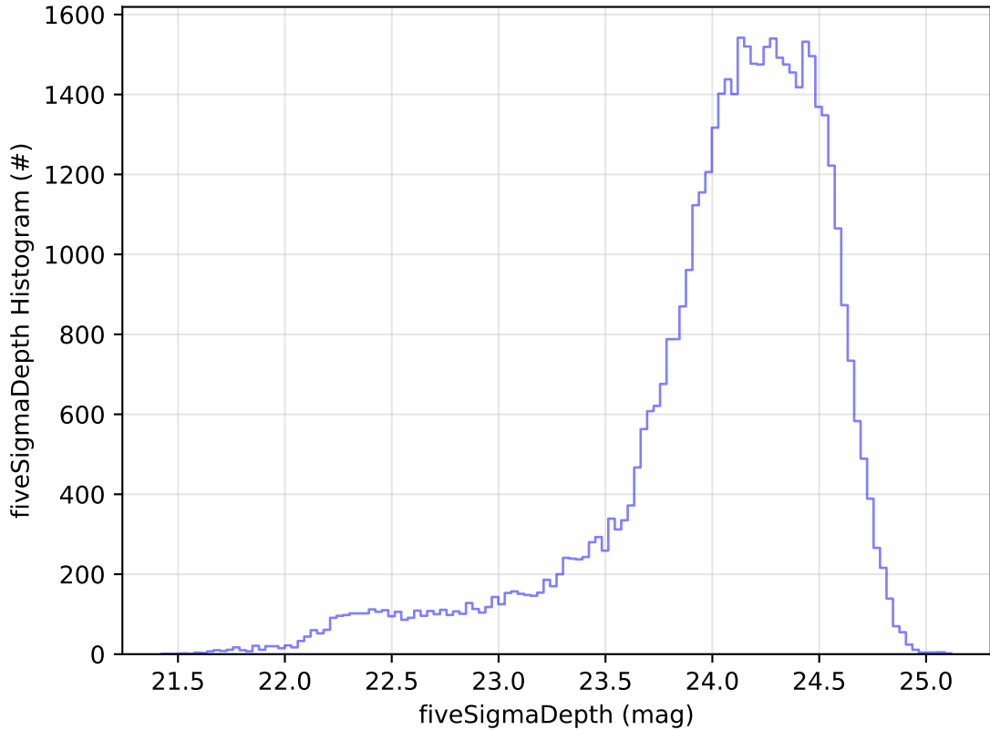
too_elab_r256_d2_ugrizy_v3.4_10yrs Yr 1 r band: fiveSigmaDepth Histogram
