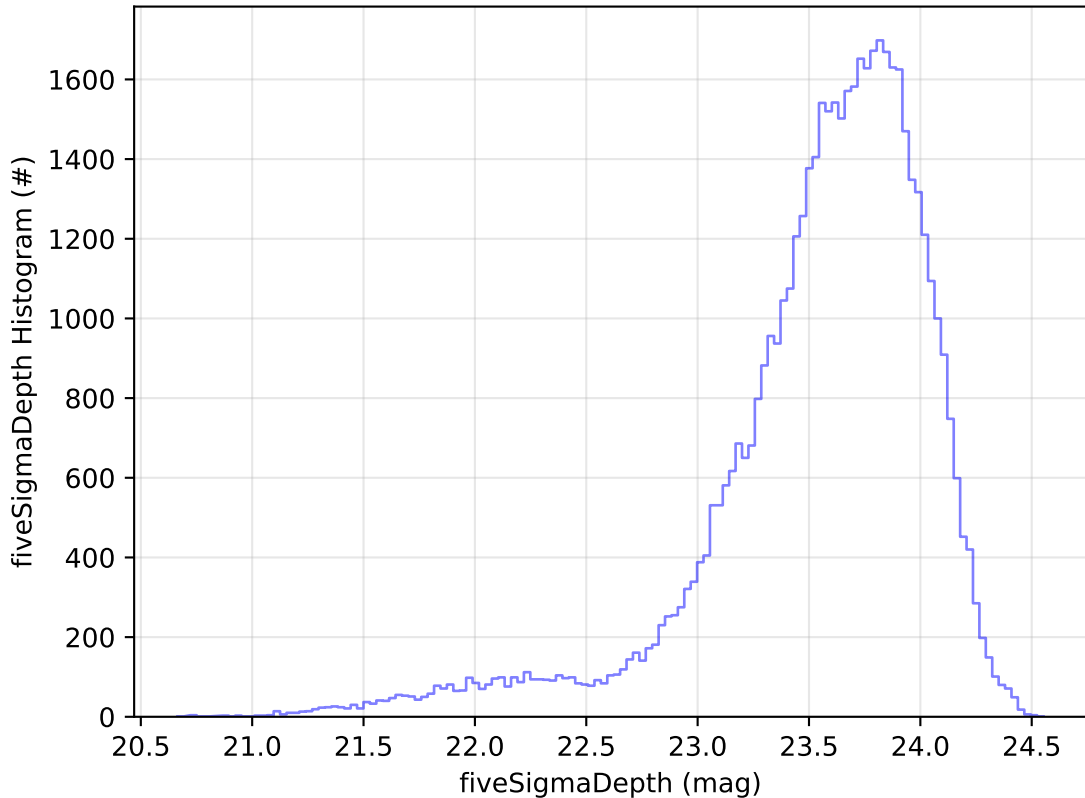
too_elab_r256_d2_ugrizy_v3.4_10yrs Yr 1 i band: fiveSigmaDepth Histogram
