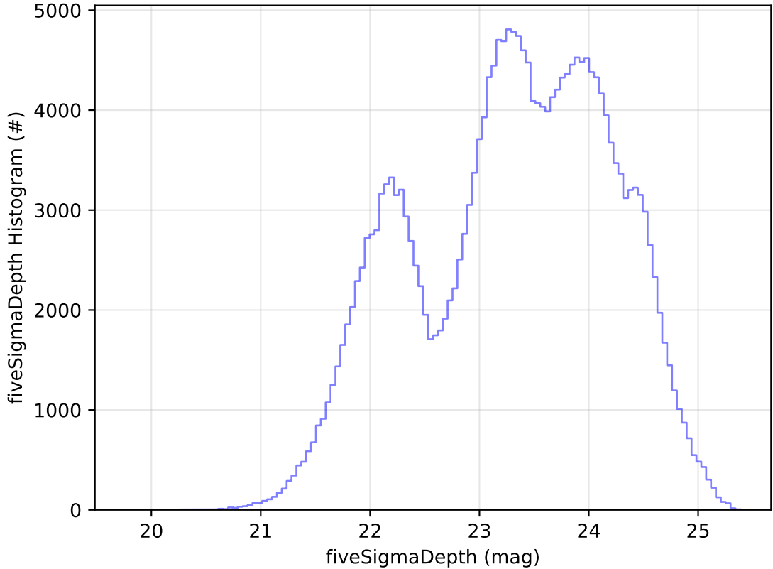
too_elab_r256_d2_ugrizy_v3.4_10yrs Yr 1 all bands: fiveSigmaDepth Histogram
