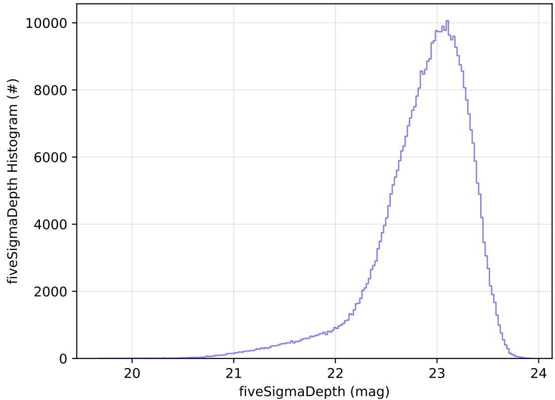
too_elab_r256_d2_ugrizy_v3.4_10yrs WFD z band: fiveSigmaDepth Histogram
