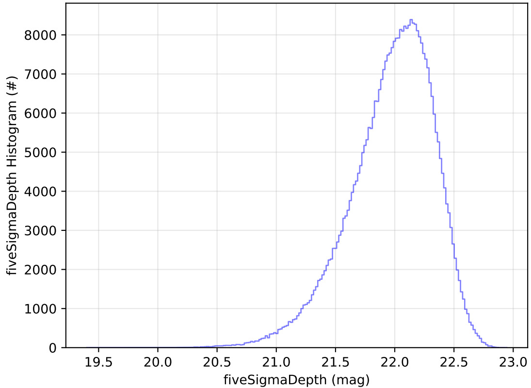
too_elab_r256_d2_ugrizy_v3.4_10yrs WFD y band: fiveSigmaDepth Histogram
