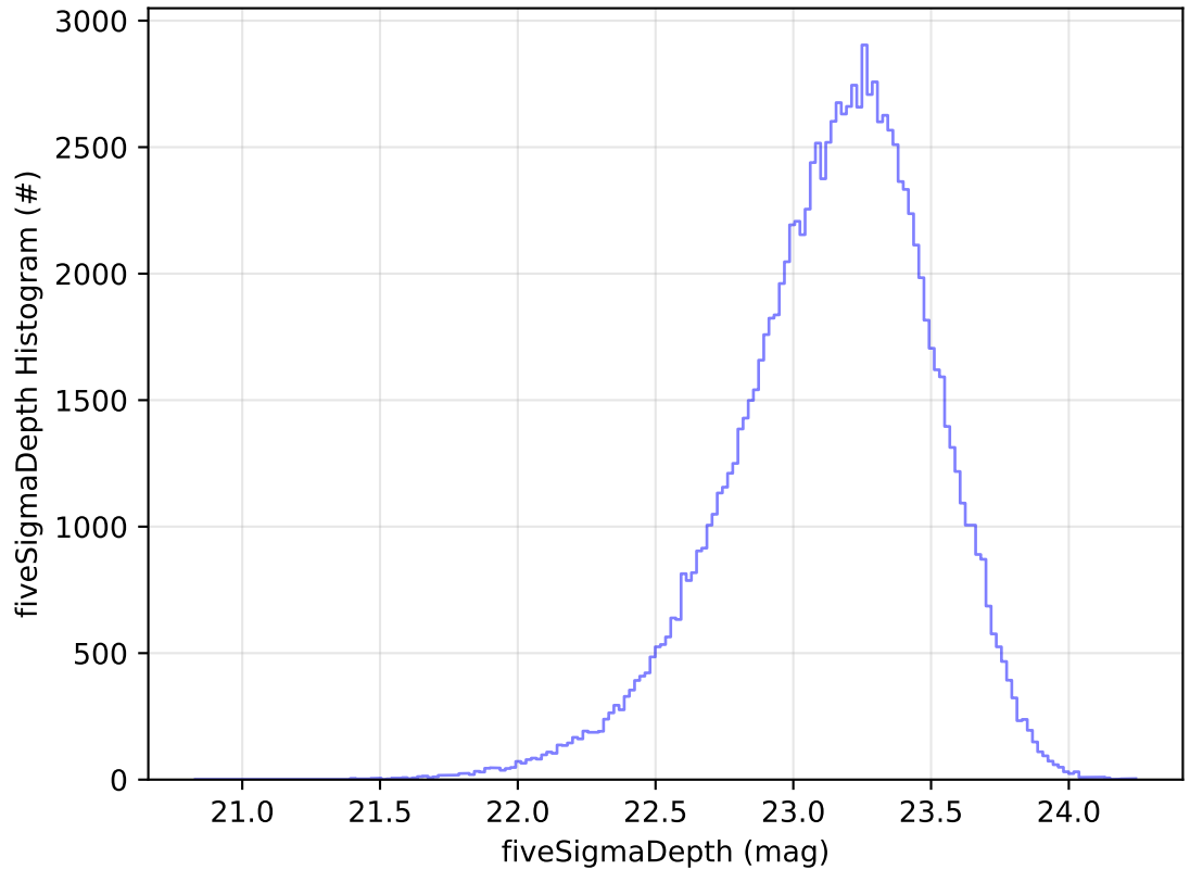
too_elab_r256_d2_ugrizy_v3.4_10yrs WFD u band: fiveSigmaDepth Histogram
