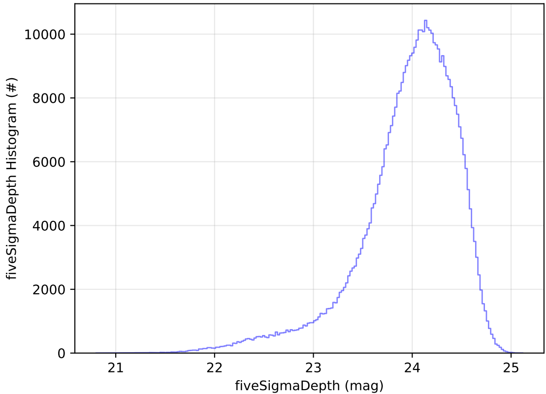
too_elab_r256_d2_ugrizy_v3.4_10yrs WFD r band: fiveSigmaDepth Histogram
