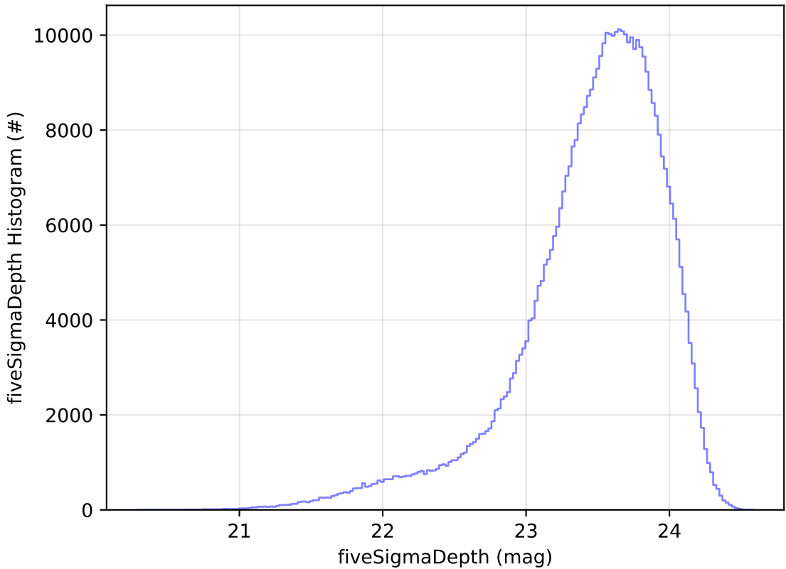
too_elab_r256_d2_ugrizy_v3.4_10yrs WFD i band: fiveSigmaDepth Histogram
