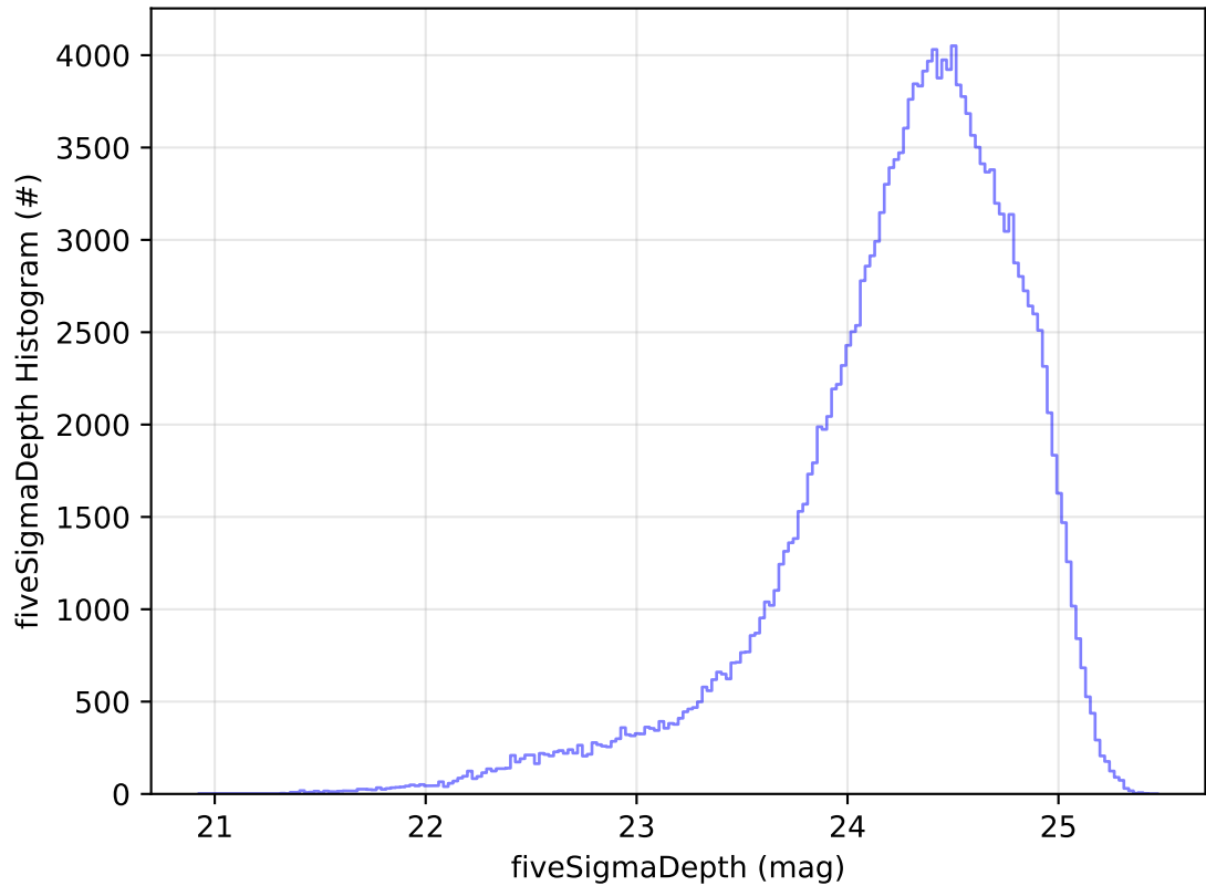
too_elab_r256_d2_ugrizy_v3.4_10yrs WFD g band: fiveSigmaDepth Histogram
