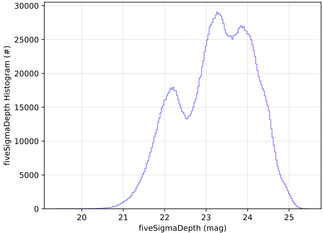
too_elab_r256_d2_ugrizy_v3.4_10yrs WFD all bands: fiveSigmaDepth Histogram
