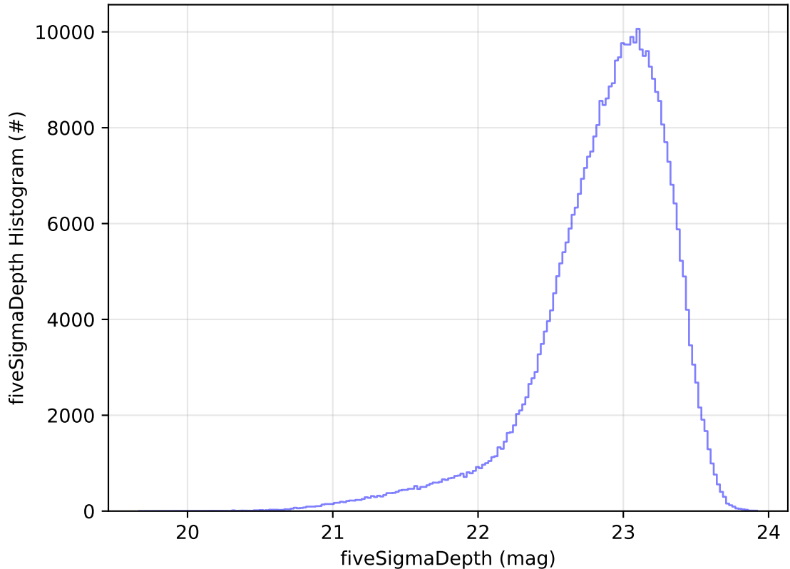
too_elab_r256_d2_ugrizy_v3.4_10yrs All sky z band: fiveSigmaDepth Histogram
