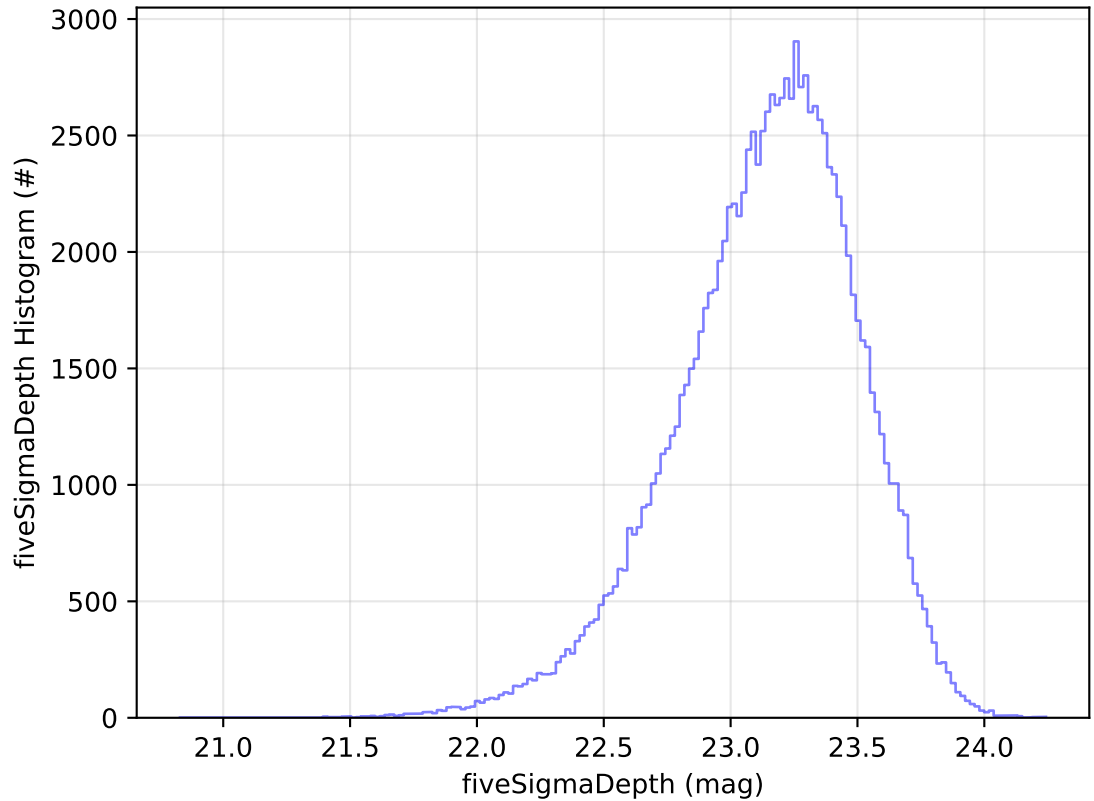
too_elab_r256_d2_ugrizy_v3.4_10yrs All sky u band: fiveSigmaDepth Histogram
