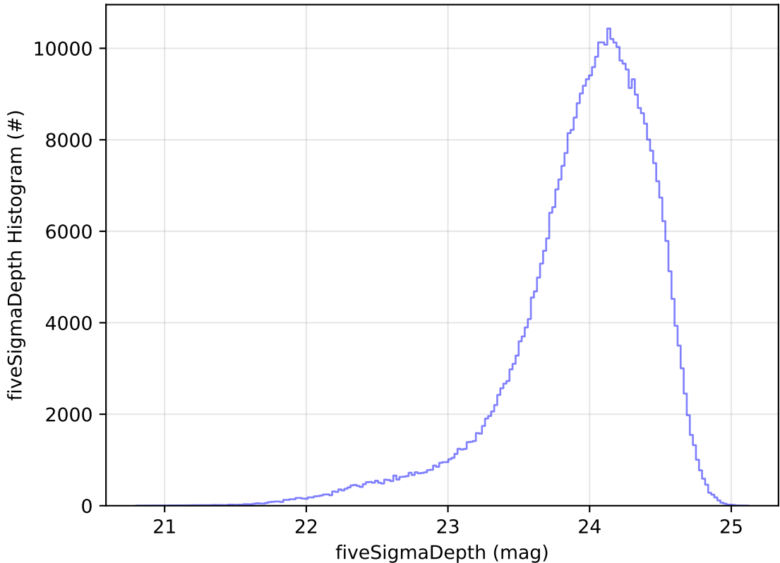
too_elab_r256_d2_ugrizy_v3.4_10yrs All sky r band: fiveSigmaDepth Histogram
