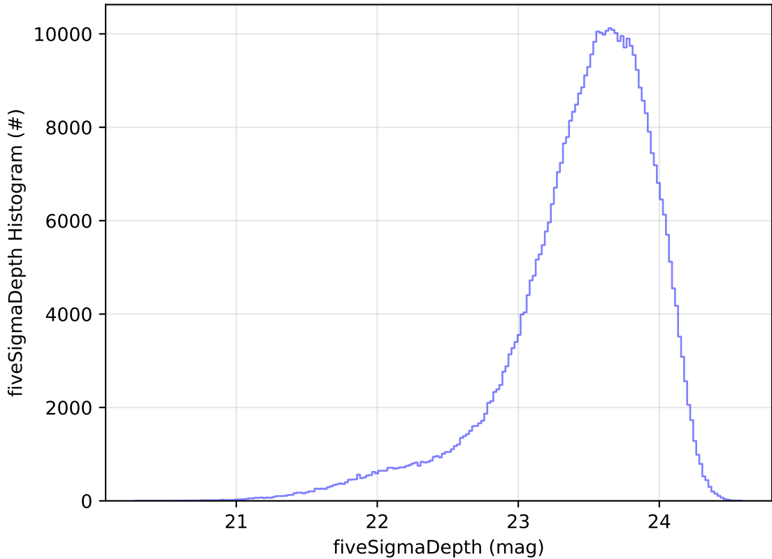
too_elab_r256_d2_ugrizy_v3.4_10yrs All sky i band: fiveSigmaDepth Histogram
