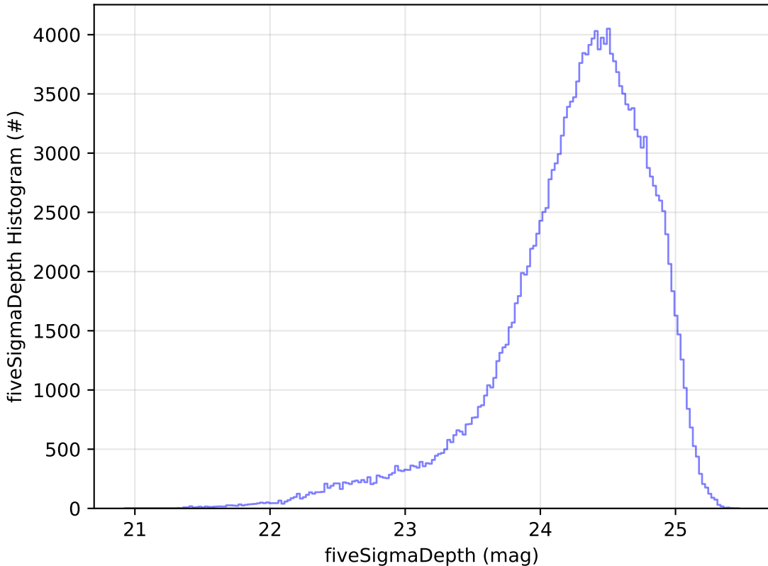
too_elab_r256_d2_ugrizy_v3.4_10yrs All sky g band: fiveSigmaDepth Histogram
