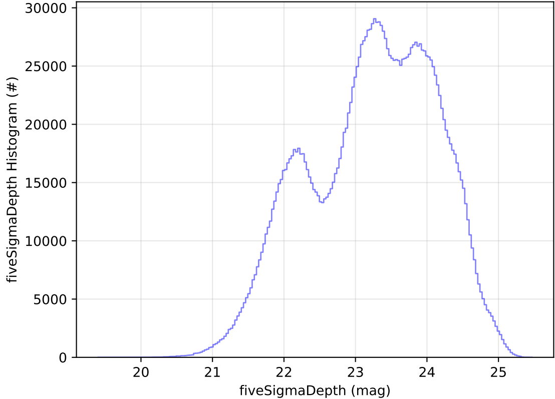
too_elab_r256_d2_ugrizy_v3.4_10yrs All sky all bands: fiveSigmaDepth Histogram
