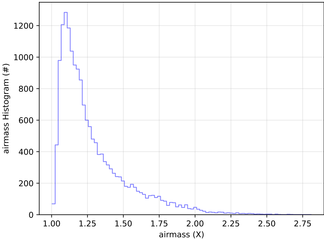
too_elab_r256_d2_ugrizy_v3.4_10yrs Yr 1 u band: airmass Histogram
