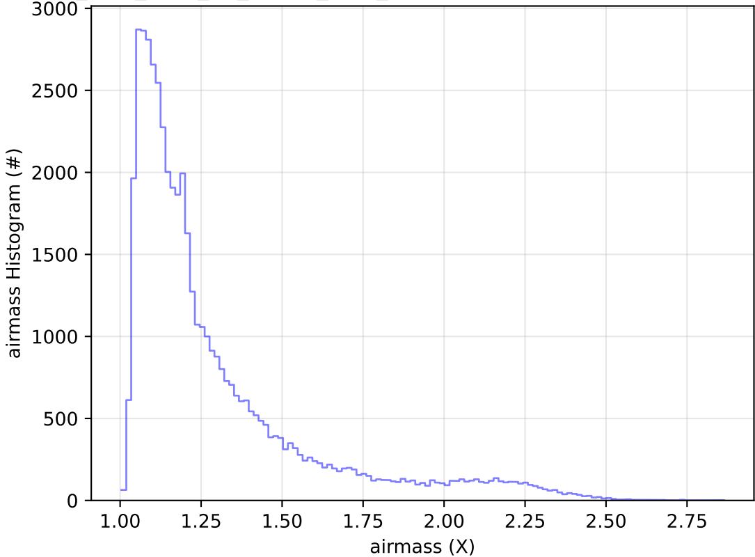
too_elab_r256_d2_ugrizy_v3.4_10yrs Yr 1 r band: airmass Histogram
