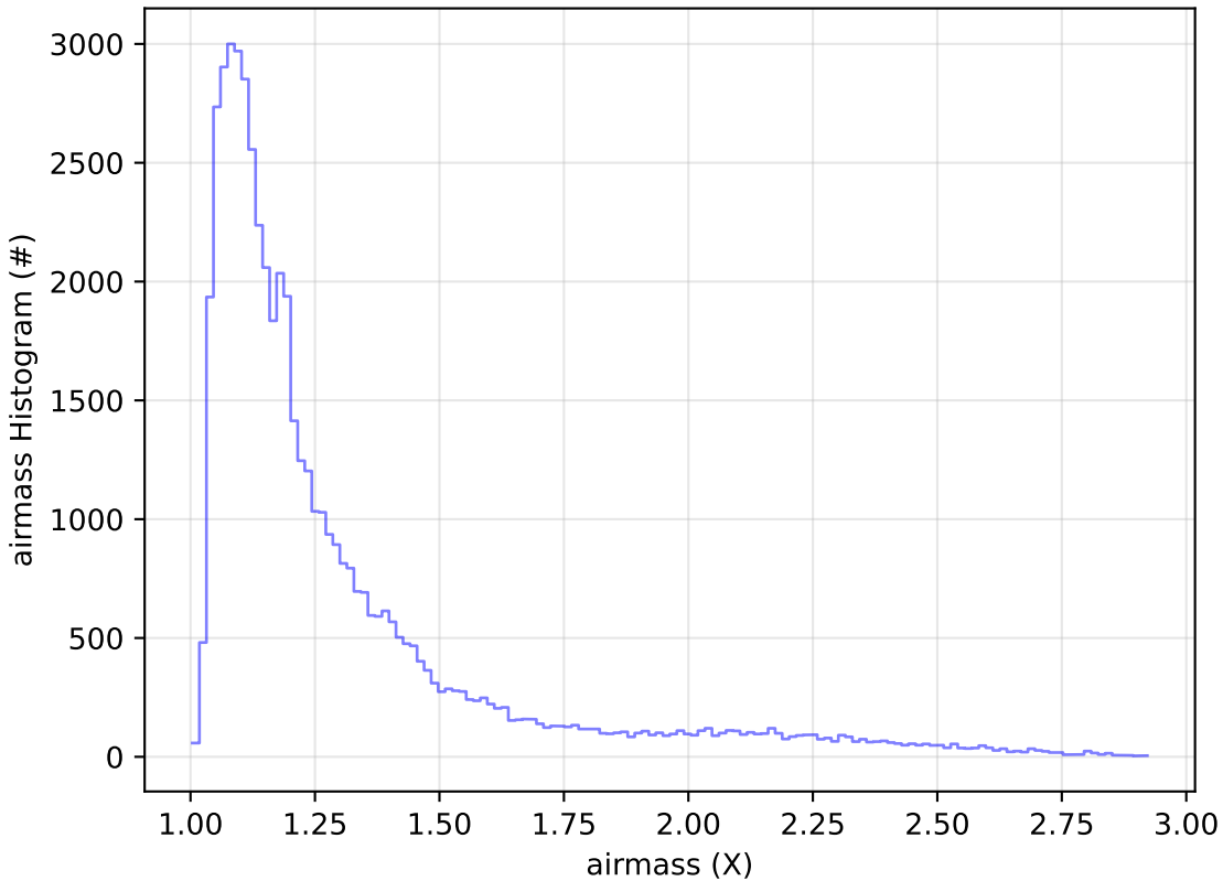
too_elab_r256_d2_ugrizy_v3.4_10yrs Yr 1 i band: airmass Histogram
