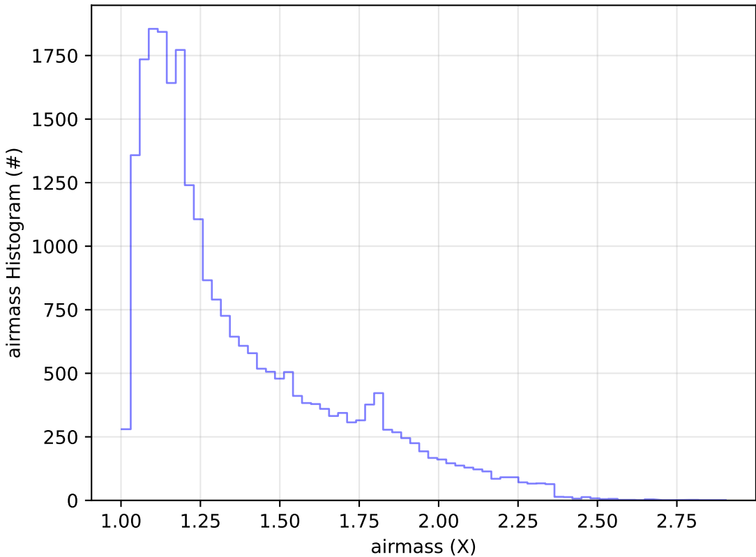
too_elab_r256_d2_ugrizy_v3.4_10yrs Yr 1 g band: airmass Histogram
