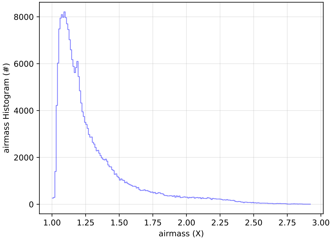
too_elab_r256_d2_ugrizy_v3.4_10yrs Yr 1 all bands: airmass Histogram
