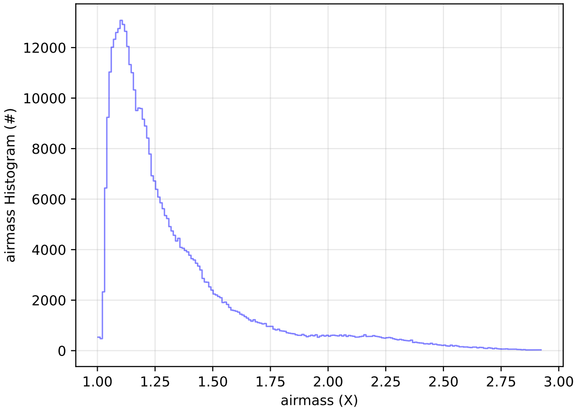
too_elab_r256_d2_ugrizy_v3.4_10yrs WFD z band: airmass Histogram
