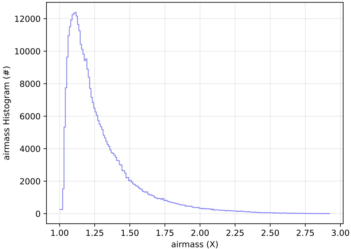
too_elab_r256_d2_ugrizy_v3.4_10yrs WFD y band: airmass Histogram
